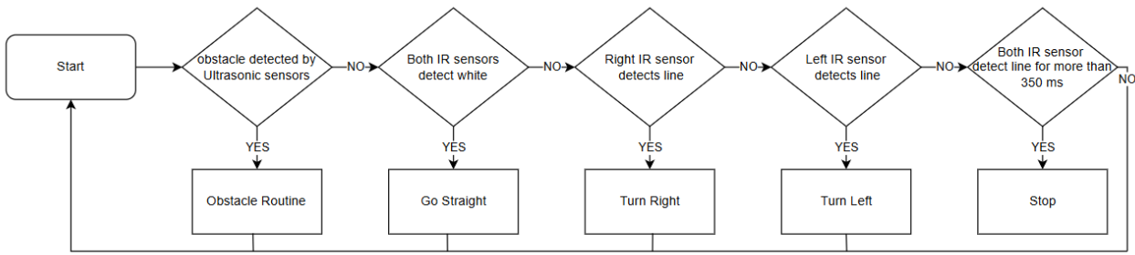
Figure 3. Line-Following control loop (§3.5). Each iteration resolves the highest priority condition first — obstacle, then line following.
